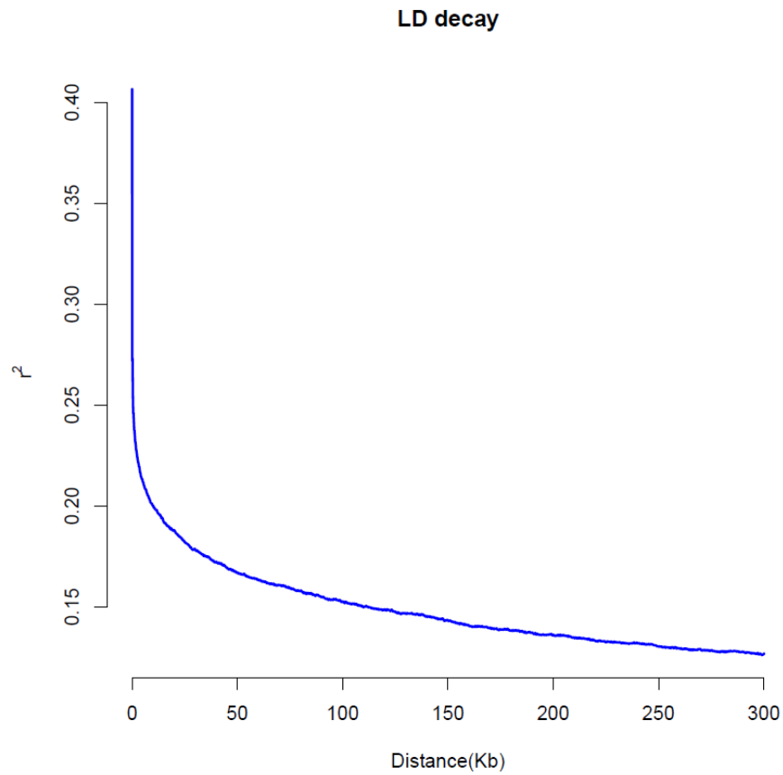
Fig. S1. LD decay analysis.
